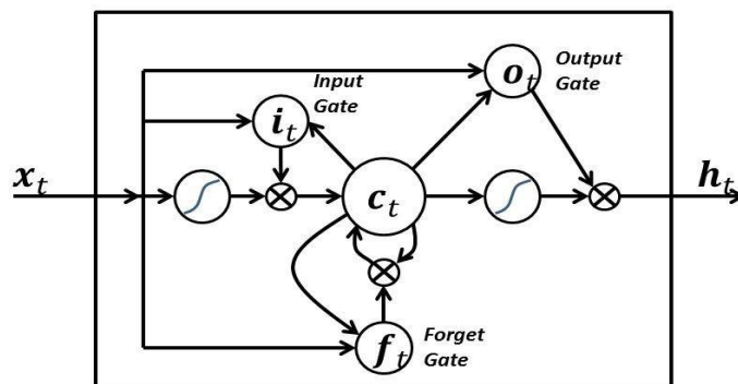
Fig. 2: Long Short-Term Memory Architecture[9].
