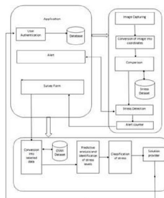
Fig.4.Architecture diagram of stress detection system
